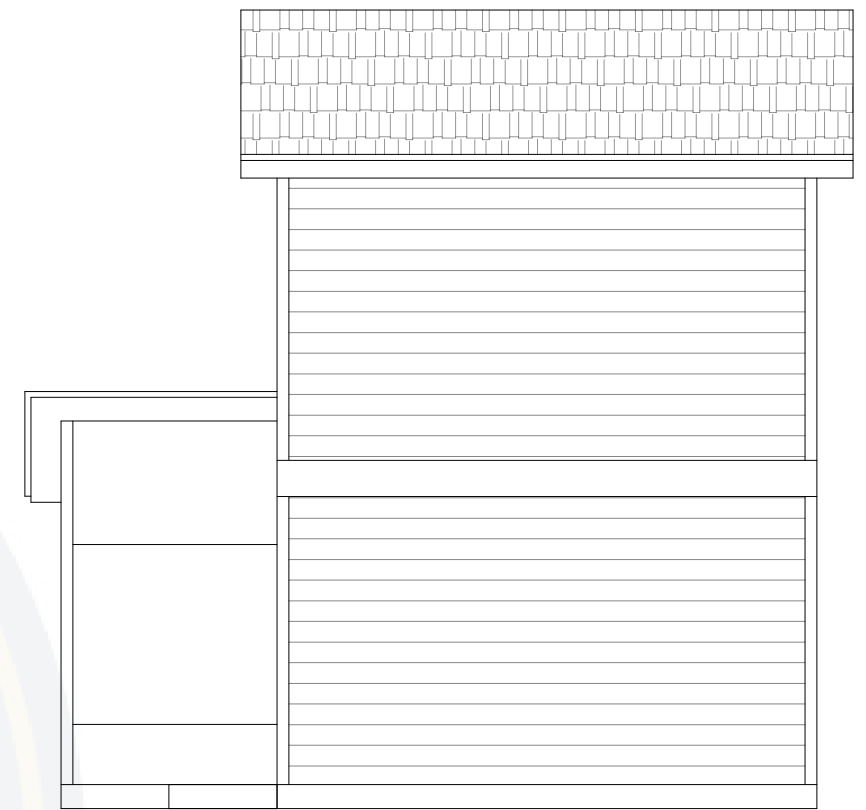
○ RIGHT ELEVATION SCALE: 3/16" = 1'-0"
