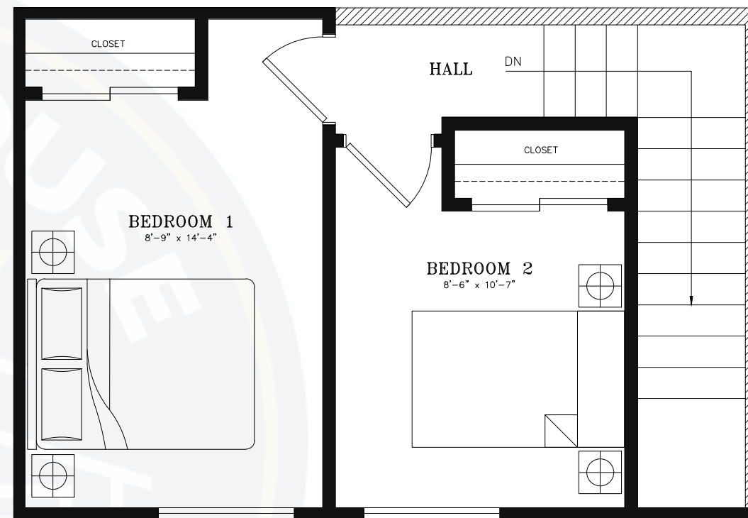
○ SECOND FLOOR PLAN 330 TOTAL SQ.FT.
