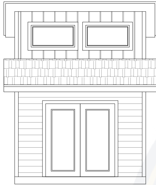
○ FRONT ELEVATION SCALE: 3/16'' = 1'-0''
