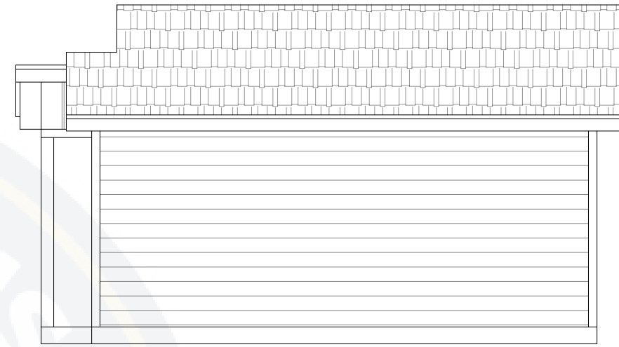
○ RIGHT ELEVATION SCALE: 3/16" = 1'-0"
