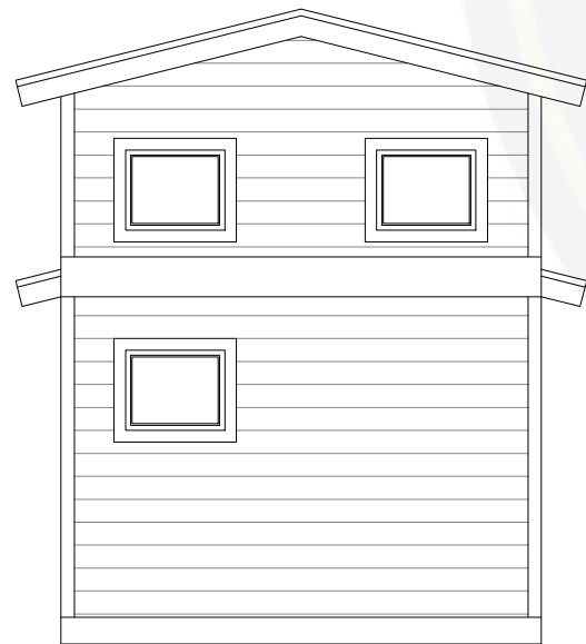
○ REAR ELEVATION SCALE: 3/16'' = 1'-0''
