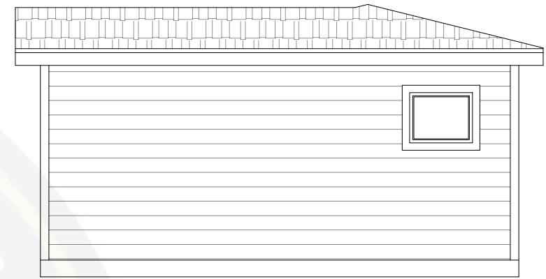
○ RIGHT ELEVATION SCALE: 3/16" = 1'-0"
